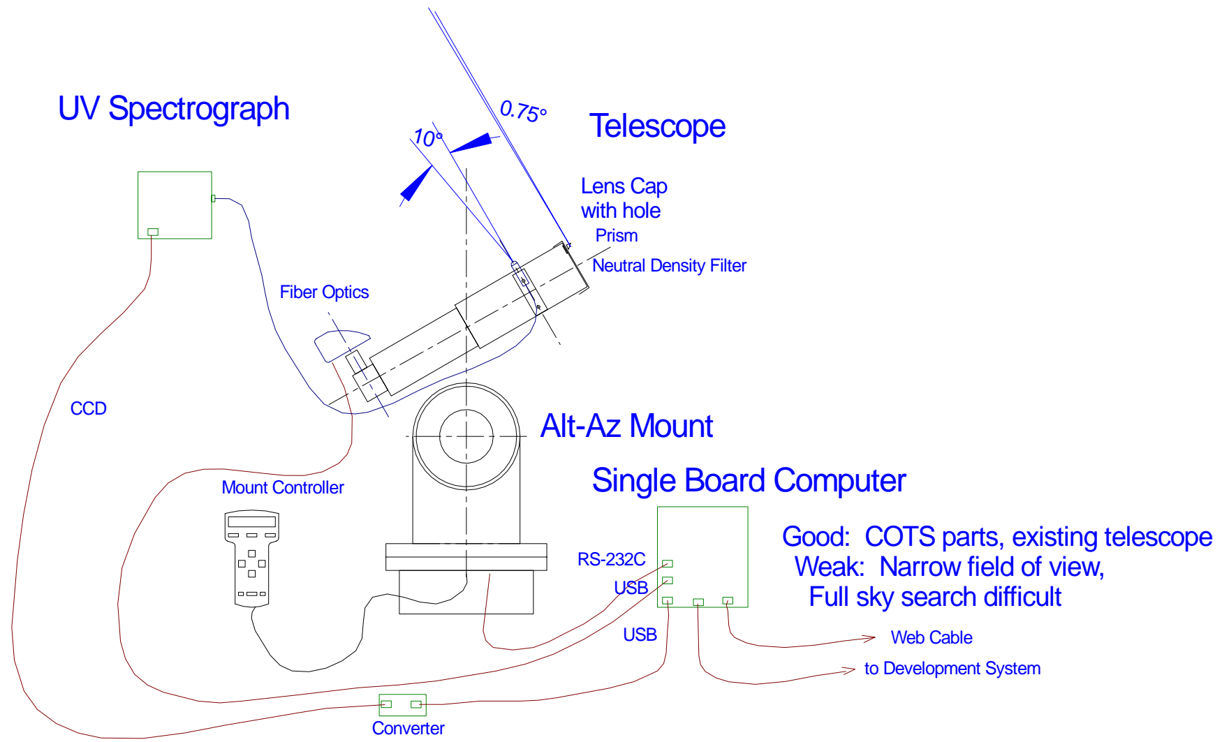
Configuration 2: CCD Tracking, Small Field of View
