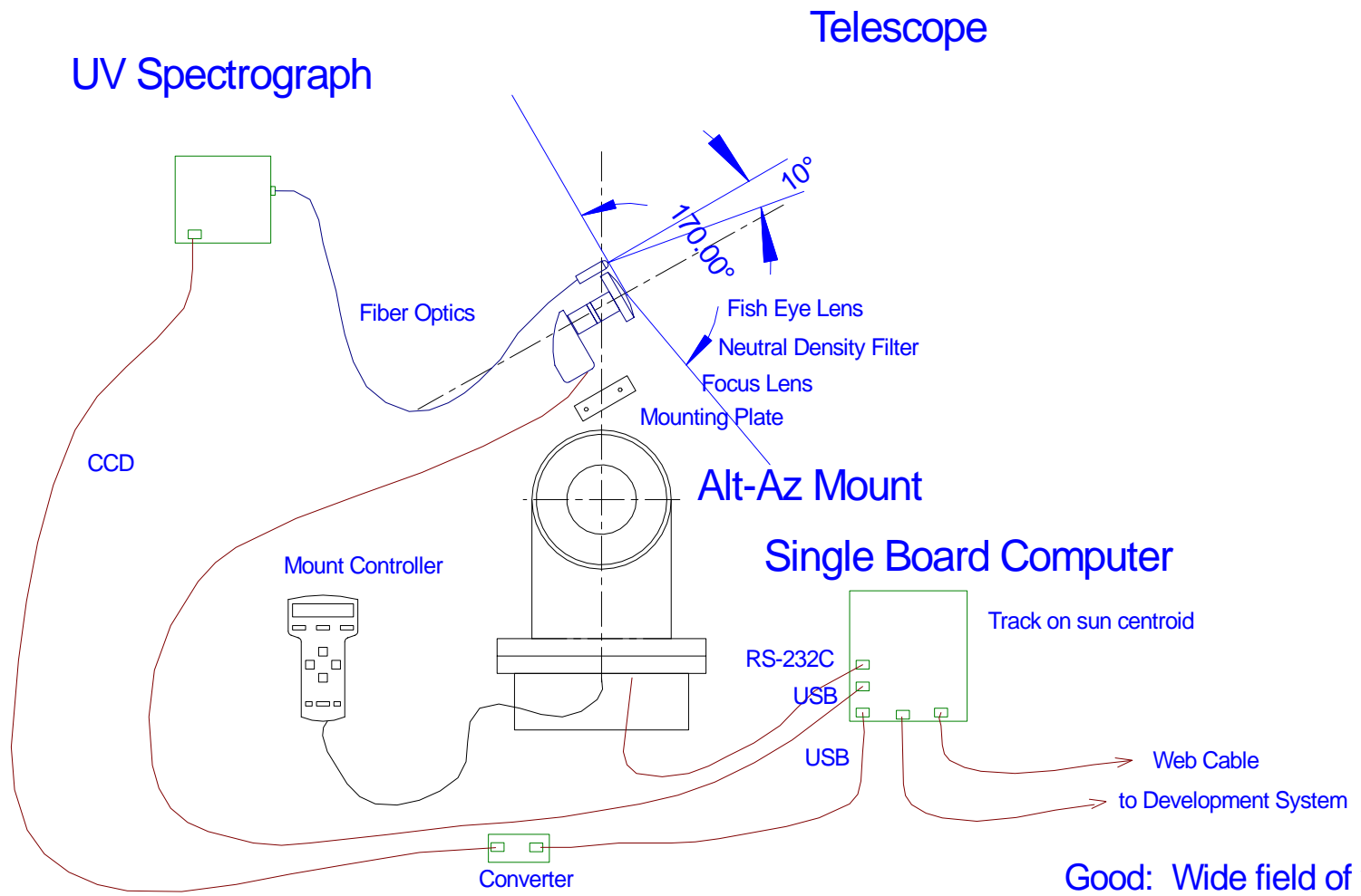
Configuration 3: CCD Tracking, Wide Field of View
