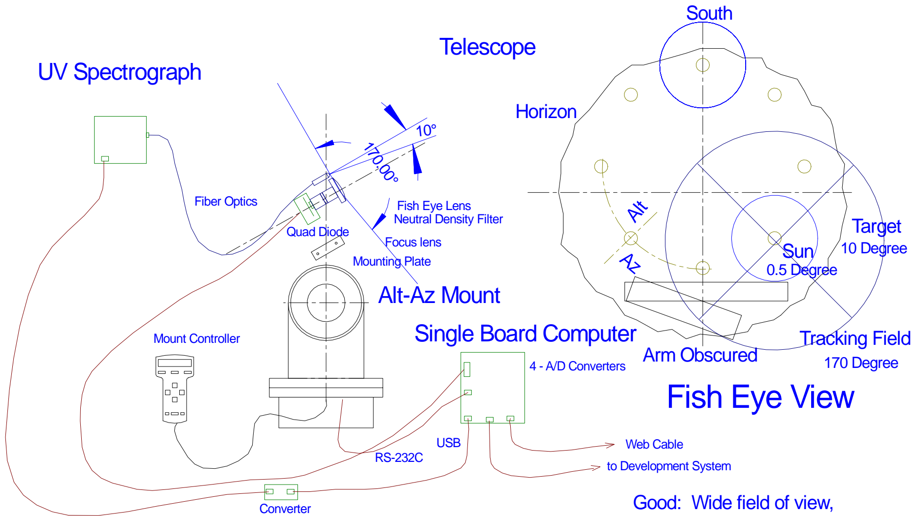
Configuration 4: Quad Diode Tracking, Wide Field of View
